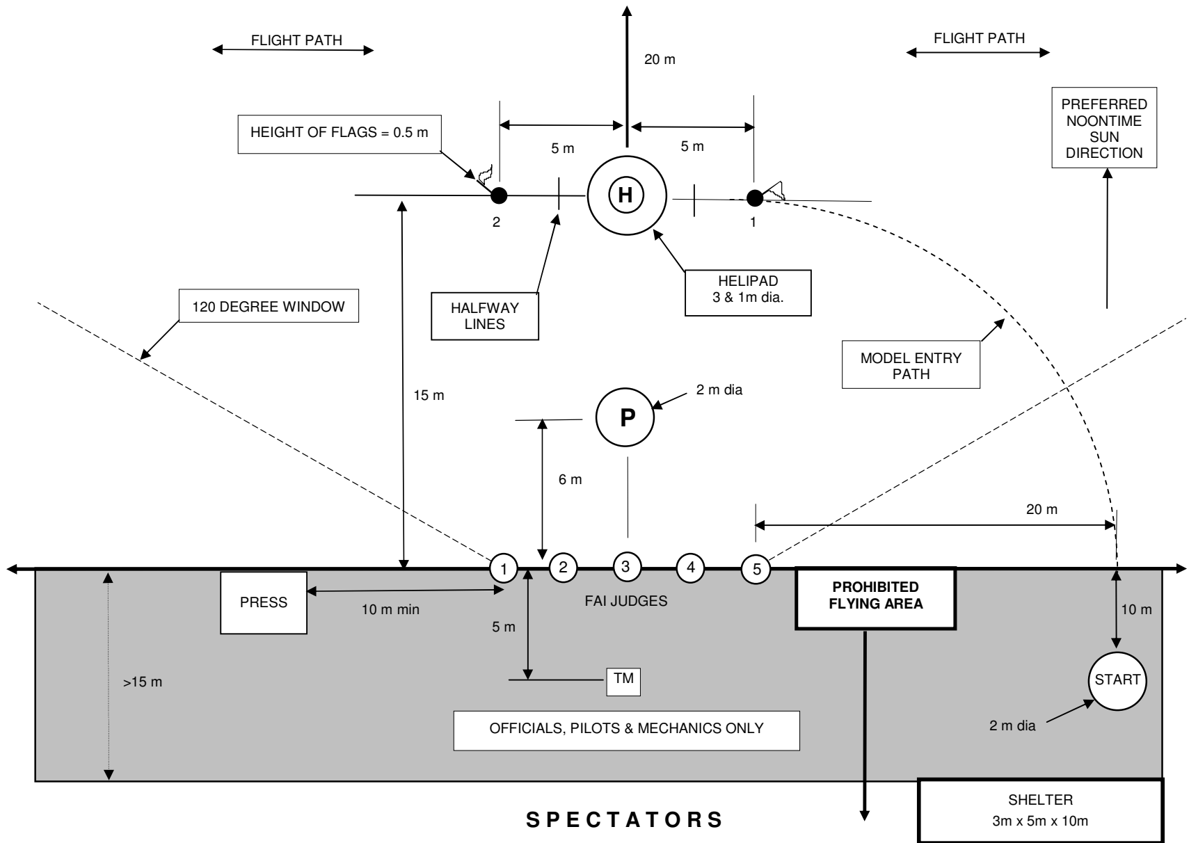
FIGURE 5.4.A - F3C CONTEST AREA LAYOUT
